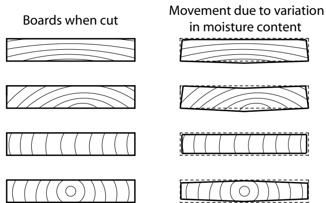
Figure 5.3 Changes in shape of boards cut from different parts of a log with changes in moisture content
