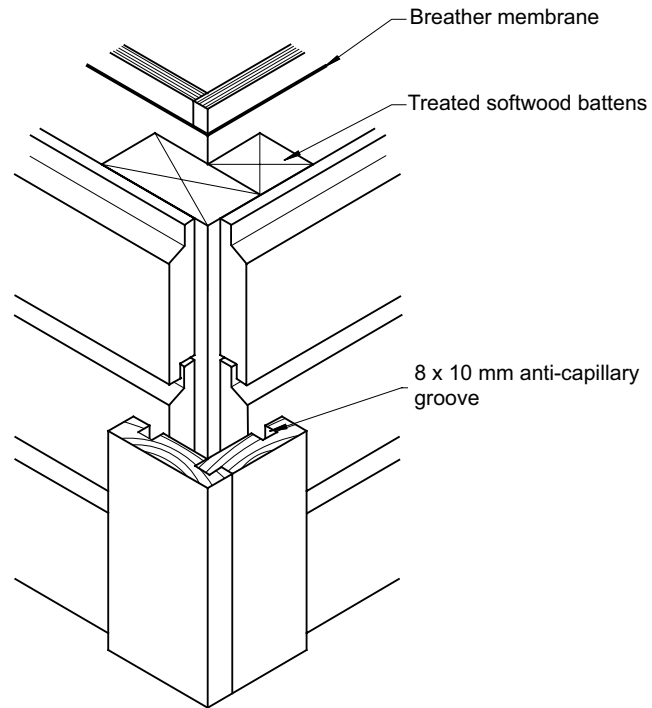
Figure 5.36 Covered corner detail in horizontal boarding
