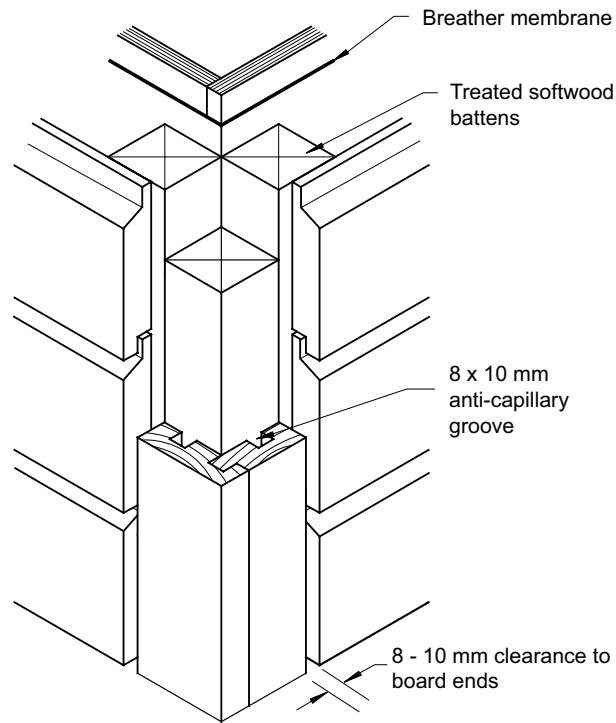
Figure 5.38 Solid corner detail in horizontal boarding with preformed capping pieces
